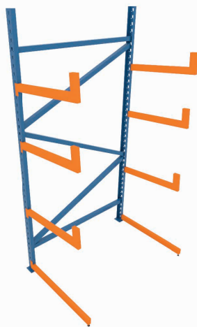
BRAZO CANTILEVER 60 CMS SOPORTE BASE 70 CMS
